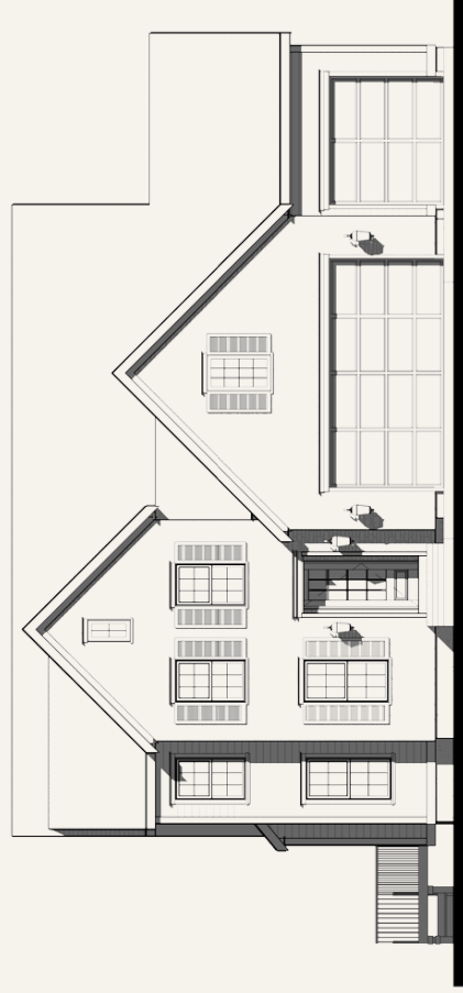
Front Elevation
